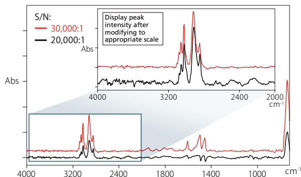
Transmission Spectra of 10 μm Diameter Polystyrene Bead Obtained by Two Infrared Microscopes AIMsight with Different Noise Levels
