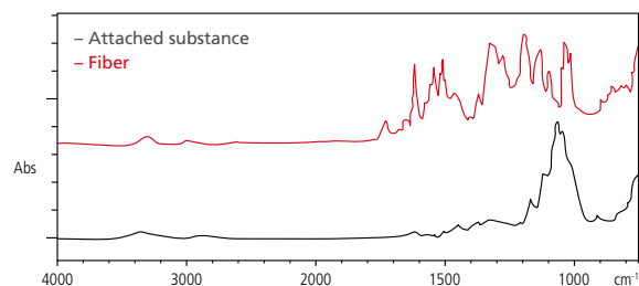
Spectrum of Substance Attached to a Fiber, Identified as a Phenol-Based Resin
