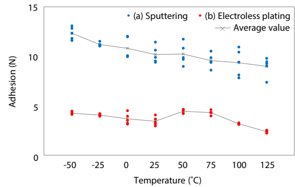
Fig. 6 Adhesion-Temperature Relationship
