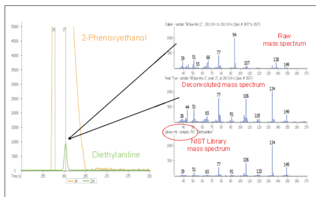
Figure 4. Automated Peak Find and spectral deconvolution for diethylaniline in the presence of 2-phenoxyethanol in a mix of blue ballpoint pen inks. Note that the raw mass spectrum taken at the peak apex for diethylaniline is characteristic of 2-phenoxyethanol due to its high concentration. The deconvoluted spectrum for diethylaniline matches well with the library spectrum.
