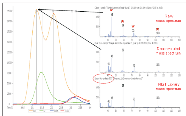
Figure 2. Automated Peak Find and spectral deconvolution for methoxy methylethoxy propanol in a blue ballpoint pen ink. The raw mass spectrum is a combination of ions (including those that are shared, marked with red asterisks) from the coelutions. The deconvoluted spectrum has a similarity of 907 (out of 999) with the library spectrum.
