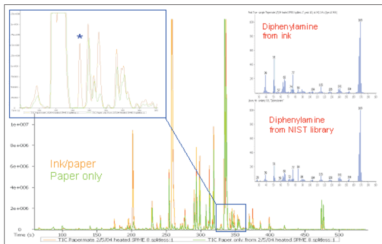
Figure 8. Overlaid TICs of paper, and paper with ink scribbles, as analyzed using SPME GC-TOFMS. Diphenylamine (blue asterisk, inset chromatogram), which was located automatically with a Compare feature of ChromaTOF, can be attributed to the ballpoint pen ink.
