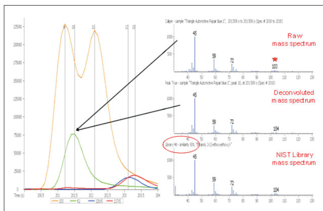
Figure 3. Automated Peak Find and spectral deconvolution for ethoxy ethoxyethanol in a blue ballpoint pen ink. The deconvoluted spectrum has a similarity of 939 (out of 999) with the library spectrum.
