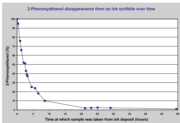
Figure 5. 2-Phenoxyethanol disappearance from an ink scribble over time as determined by SPME and fast GC-TOFMS. The concentration of 2-phenoxyethanol that can be determined by SPME GC-TOFMS stabilizes after about 20 hours.
