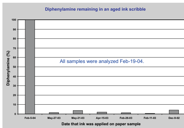
Figure 7. Diphenylamine disappearance from aged ink scribbles as determined by SPME and fast GC-TOFMS. The SPME vial was heated to 70°C prior to sampling. Diphenylamine concentration differences as determined by SPME GC-TOFMS are indistinguishable for 2003 and 2002 samples.
