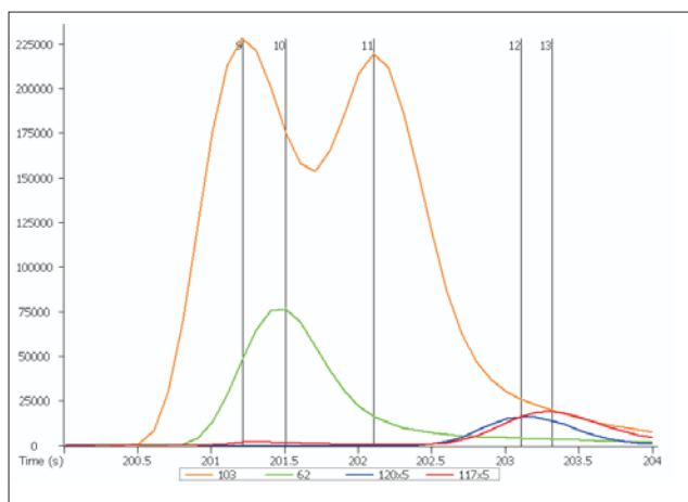
Figure 1. Automated Peak Find with ChromaTOF. Each numbered vertical line is a peak marker. Even though there are obvious coelutions, ChromaTOF located the peaks.
